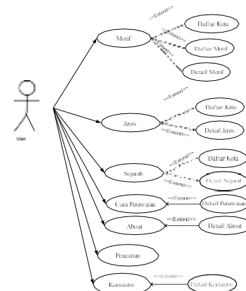
Gambar 3.1 Use Case Diagram
